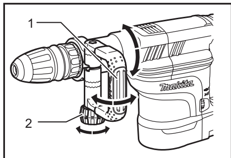
► 1. D-shaped side handle 2. Clamp nut
